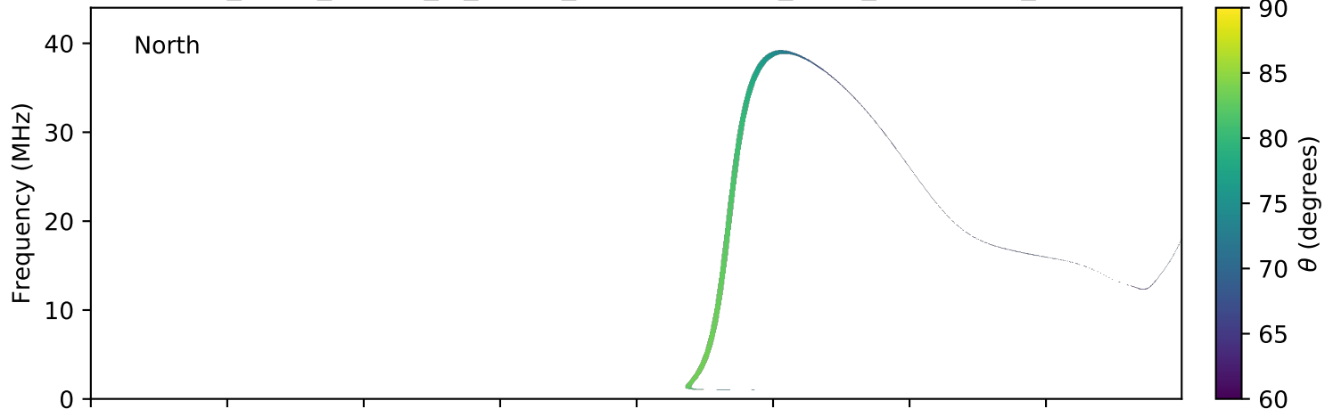
expres_earth_jupiter_io_jrm09_lossc-wid1deg_3kev_20181125_v01.cdf
