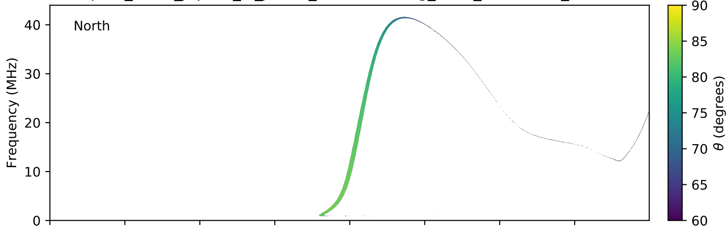
expres_earth_jupiter_io_jrm09_lossc-wid1deg_3kev_20181118_v01.cdf
