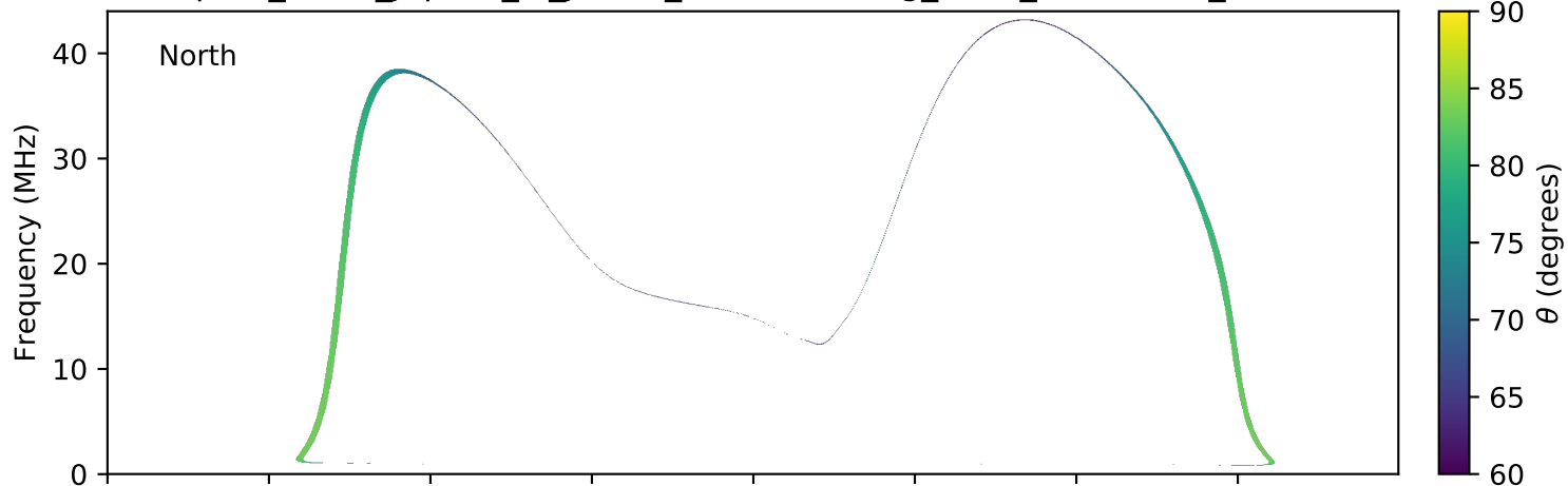
expres_earth_jupiter_io_jrm09_lossc-wid1deg_3kev_20181113_v01.cdf
