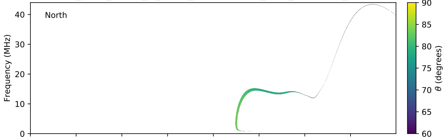
expres_earth_jupiter_io_jrm09_lossc-wid1deg_3kev_20181109_v01.cdf
