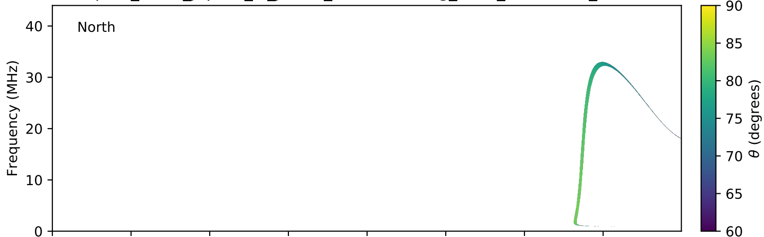
expres_earth_jupiter_io_jrm09_lossc-wid1deg_3kev_20181107_v01.cdf
