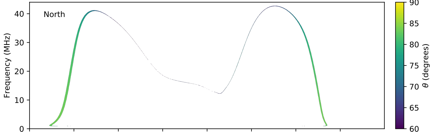
expres_earth_jupiter_io_jrm09_lossc-wid1deg_3kev_20181106_v01.cdf
