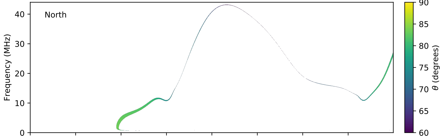
expres_earth_jupiter_io_jrm09_lossc-wid1deg_3kev_20181104_v01.cdf
