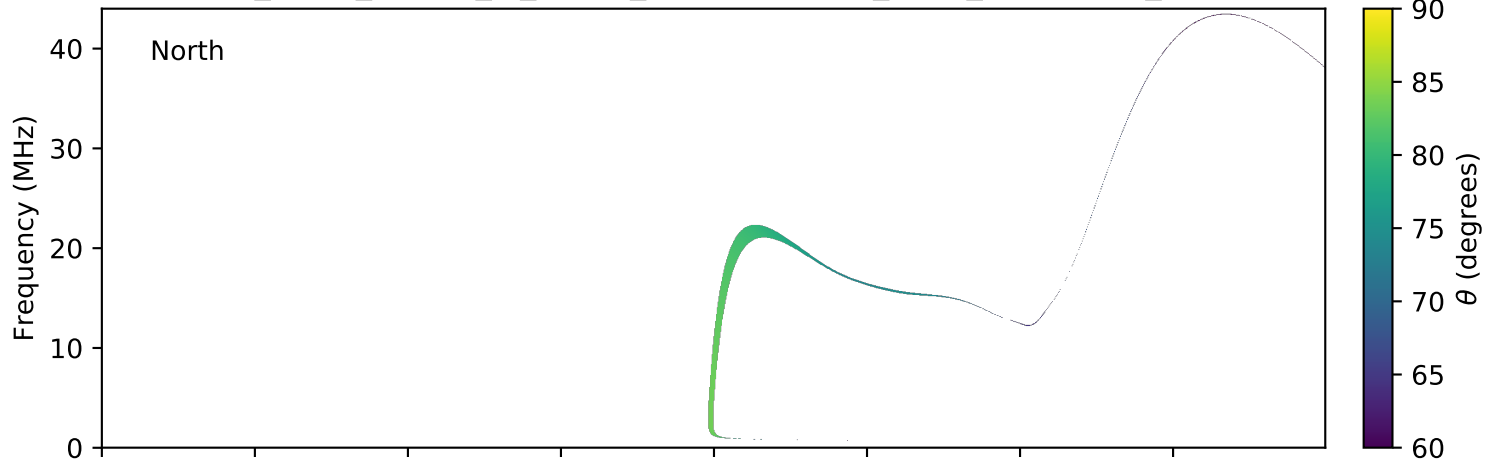
expres_earth_jupiter_io_jrm09_lossc-wid1deg_3kev_20181102_v01.cdf
