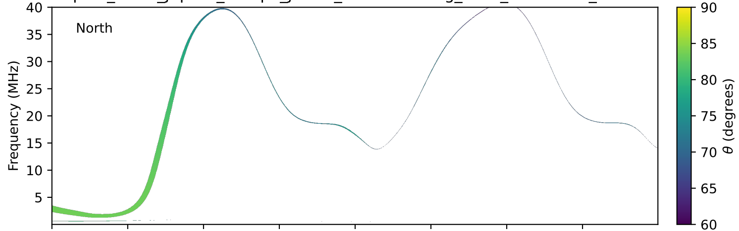
expres_earth_jupiter_europa_jrm33_lossc-wid1deg_3kev_20181108_v11.cdf
