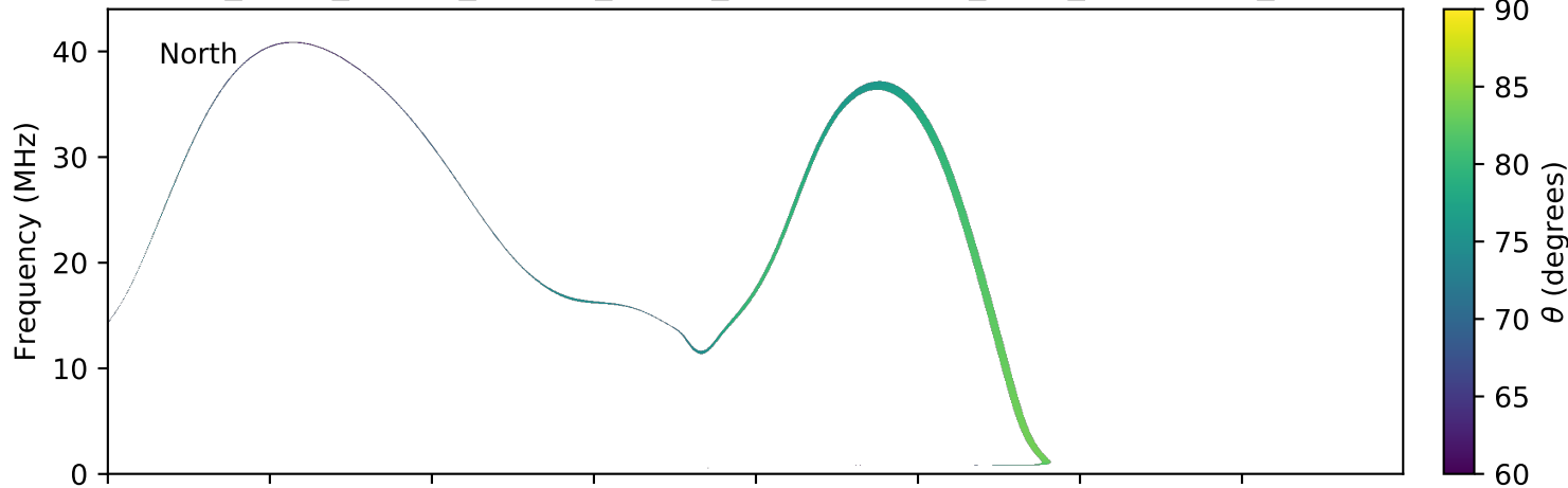
expres_earth_jupiter_europa_jrm09_lossc-wid1deg_3kev_20181121_v01.cdf
