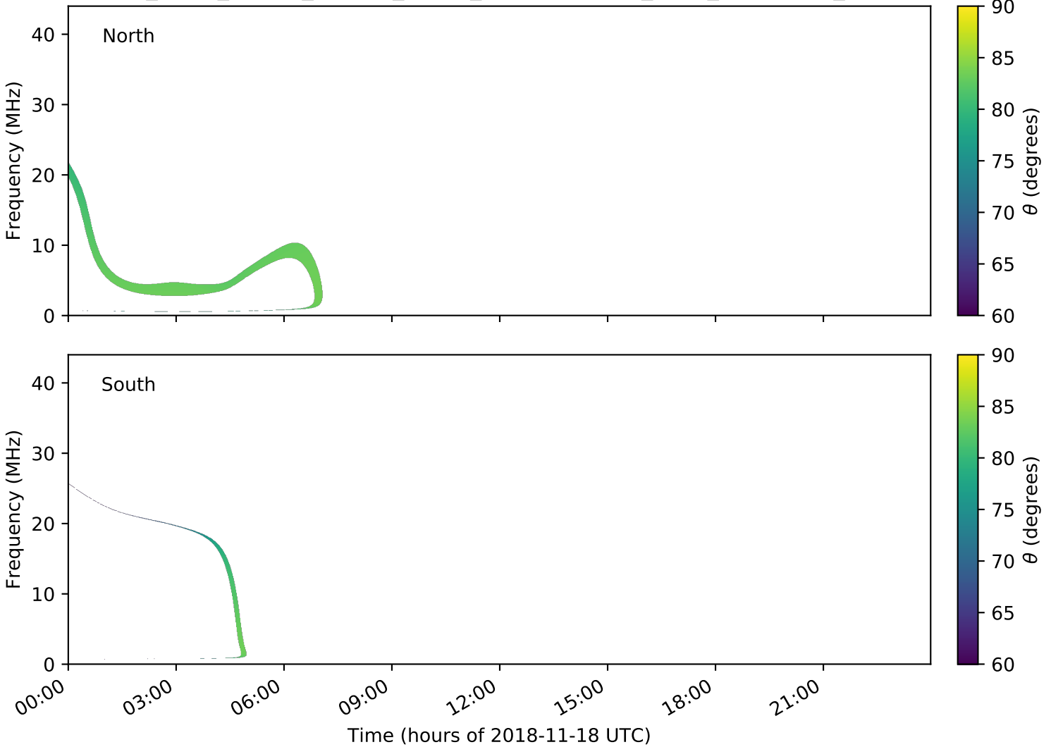
expres_earth_jupiter_europa_jrm09_lossc-wid1deg_3kev_20181118_v01.cdf
