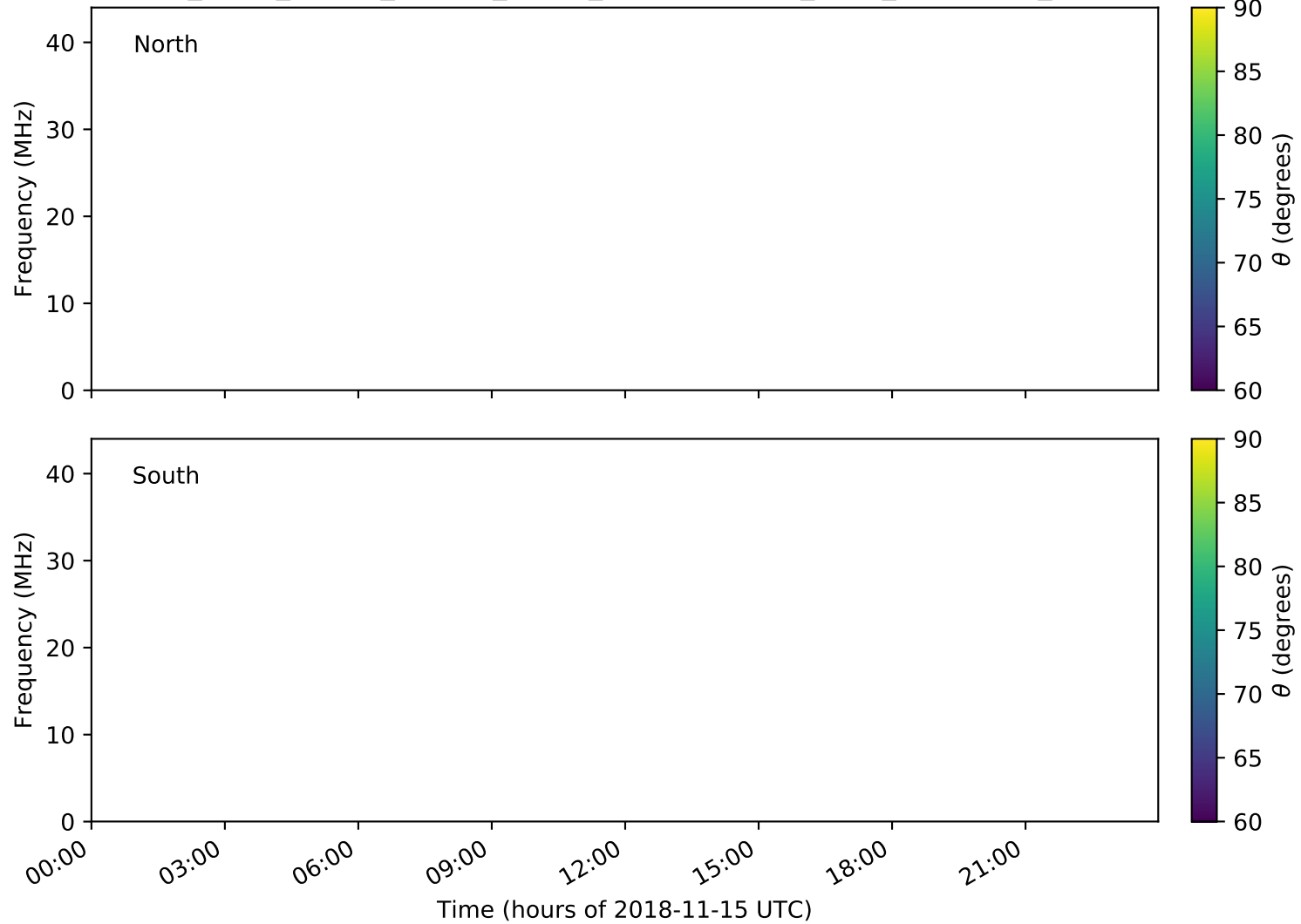
expres_earth_jupiter_europa_jrm09_lossc-wid1deg_3kev_20181115_v01.cdf
