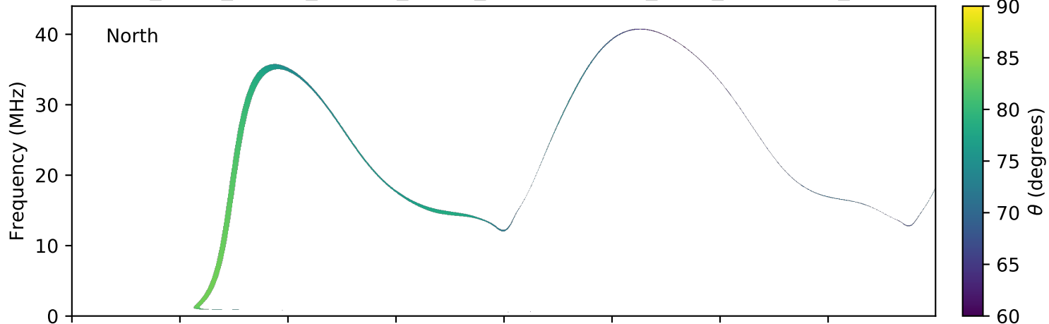
expres_earth_jupiter_europa_jrm09_lossc-wid1deg_3kev_20181113_v01.cdf
