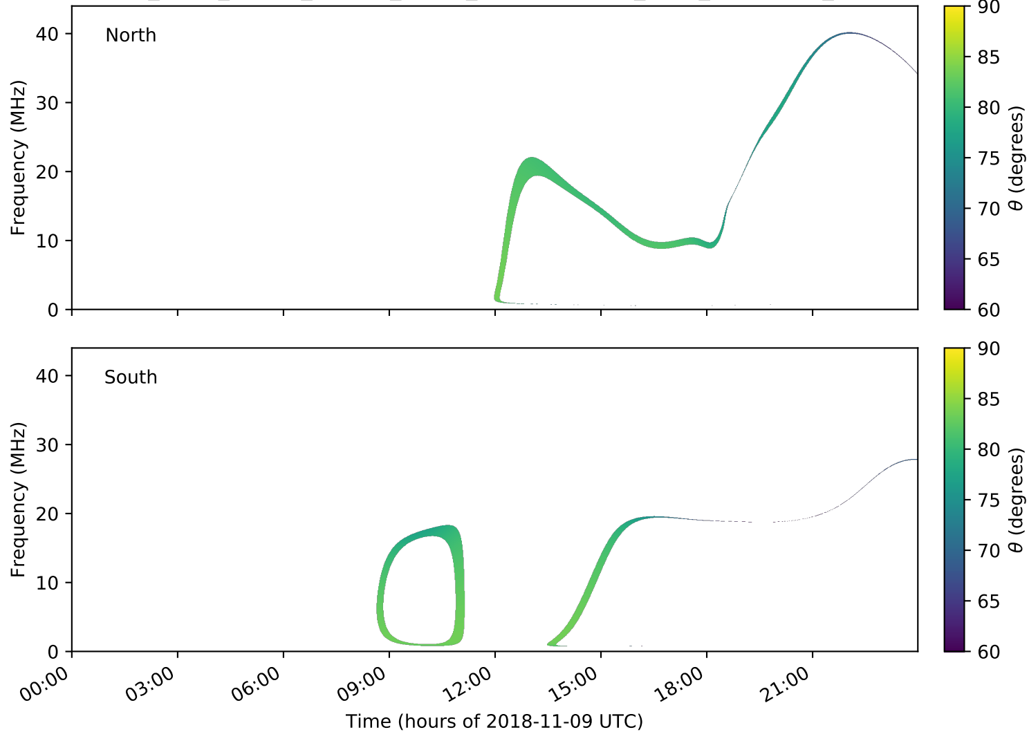
expres_earth_jupiter_europa_jrm09_lossc-wid1deg_3kev_20181109_v01.cdf
