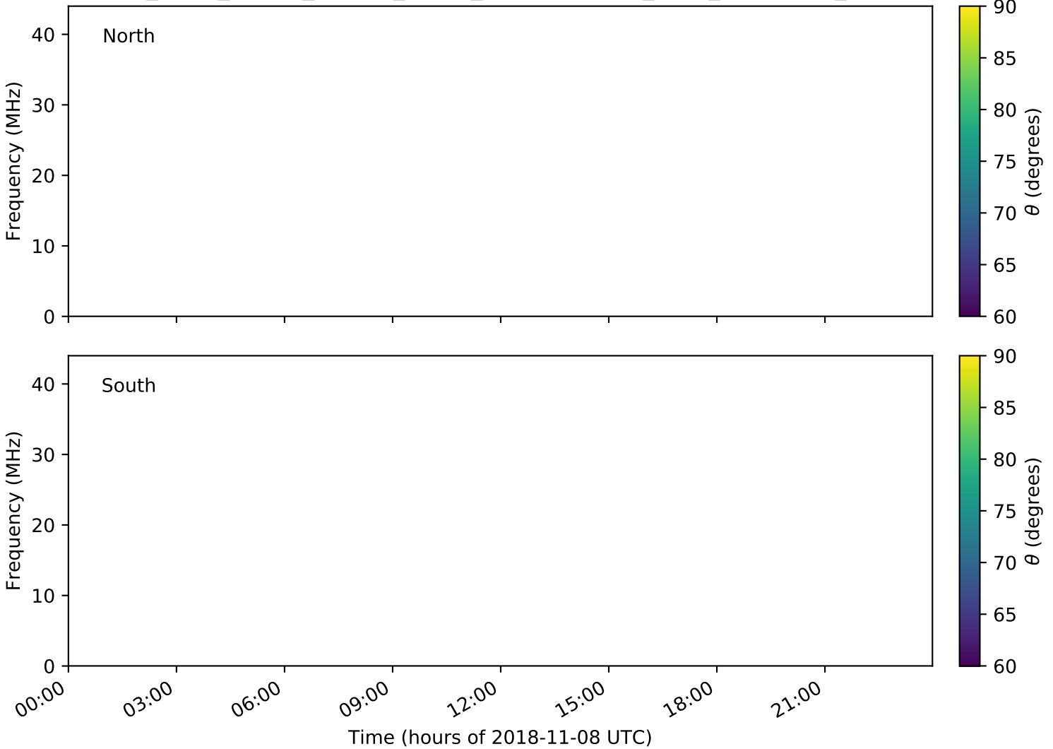
expres_earth_jupiter_europa_jrm09_lossc-wid1deg_3kev_20181108_v01.cdf
