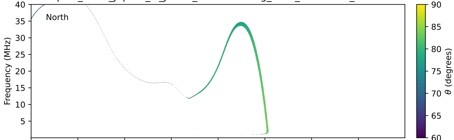
expres_earth_jupiter_io_jrm33_lossc-wid1deg_3kev_20181021_v11.cdf
