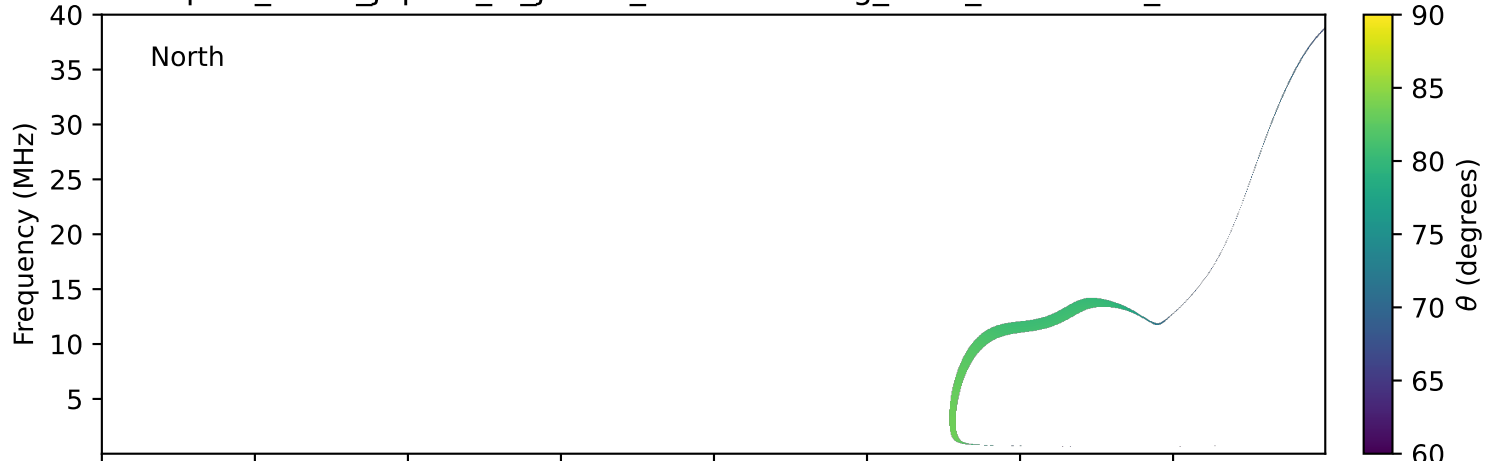
expres_earth_jupiter_io_jrm33_lossc-wid1deg_3kev_20181013_v11.cdf
