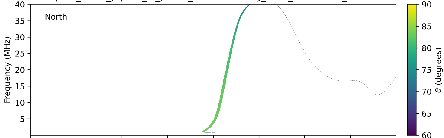
expres_earth_jupiter_io_jrm33_lossc-wid1deg_3kev_20181001_v11.cdf
