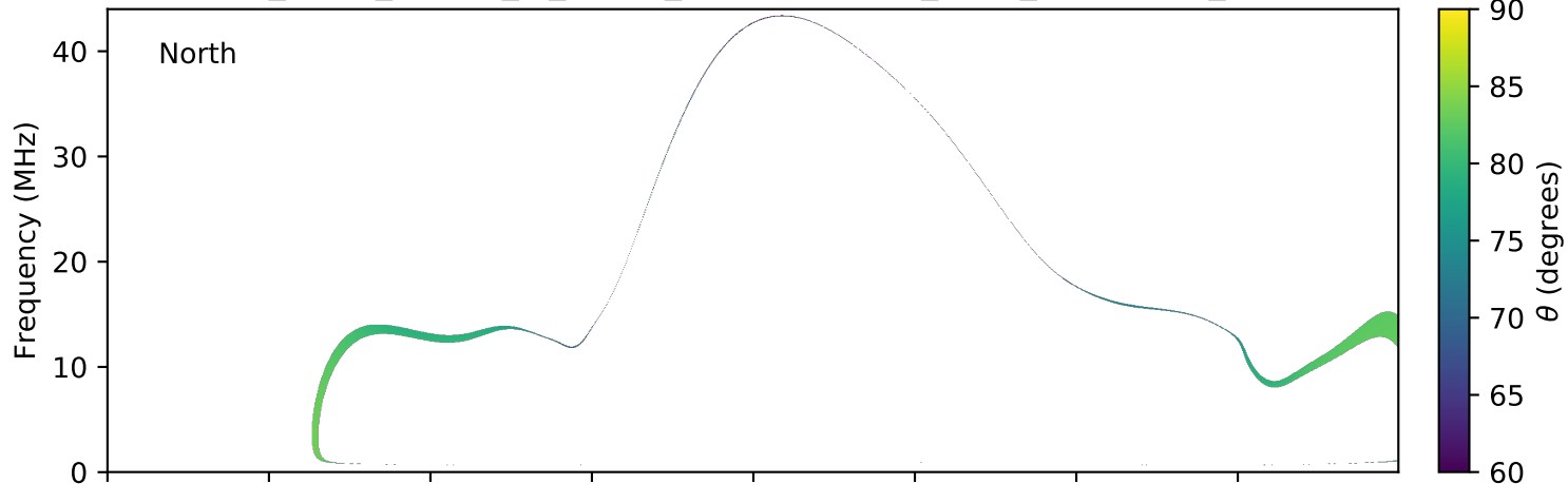
expres_earth_jupiter_io_jrm09_lossc-wid1deg_3kev_20181028_v01.cdf
