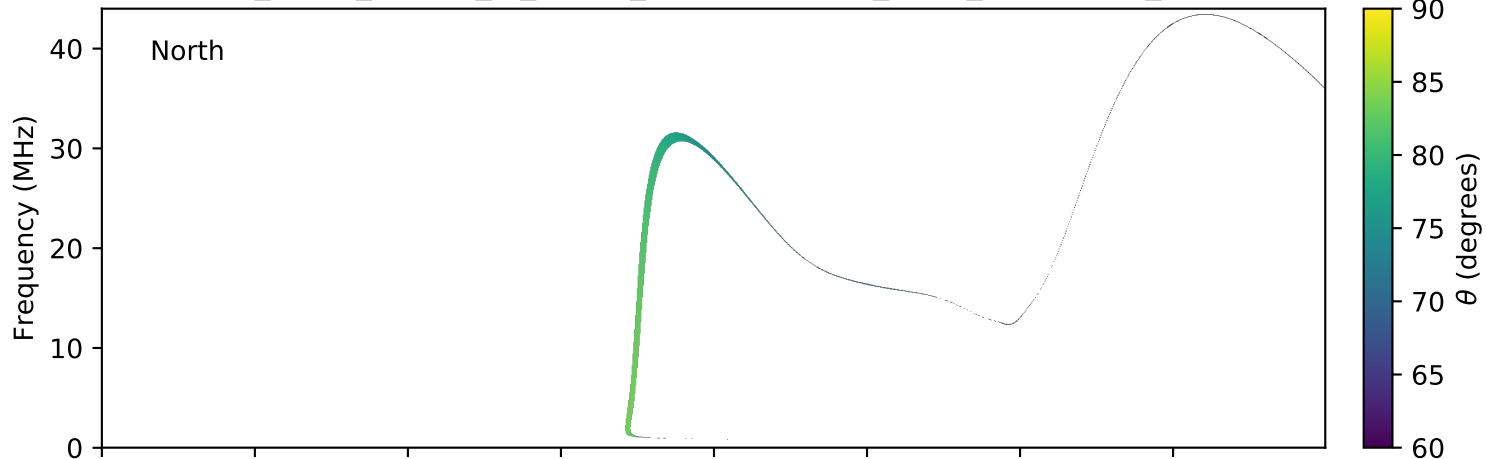
expres_earth_jupiter_io_jrm09_lossc-wid1deg_3kev_20181026_v01.cdf
