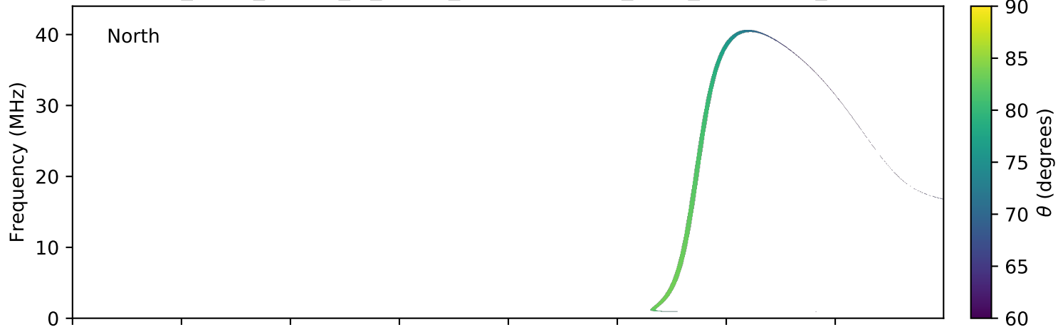
expres_earth_jupiter_io_jrm09_lossc-wid1deg_3kev_20181024_v01.cdf
