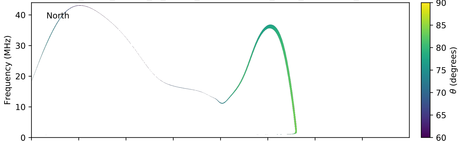
expres_earth_jupiter_io_jrm09_lossc-wid1deg_3kev_20181023_v01.cdf
