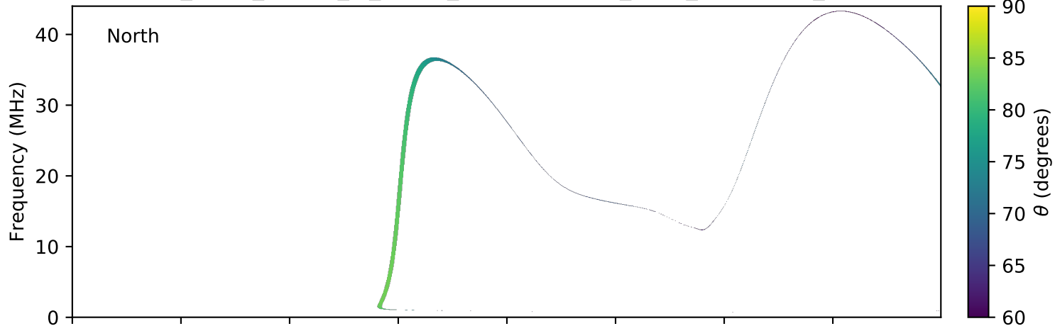
expres_earth_jupiter_io_jrm09_lossc-wid1deg_3kev_20181019_v01.cdf
