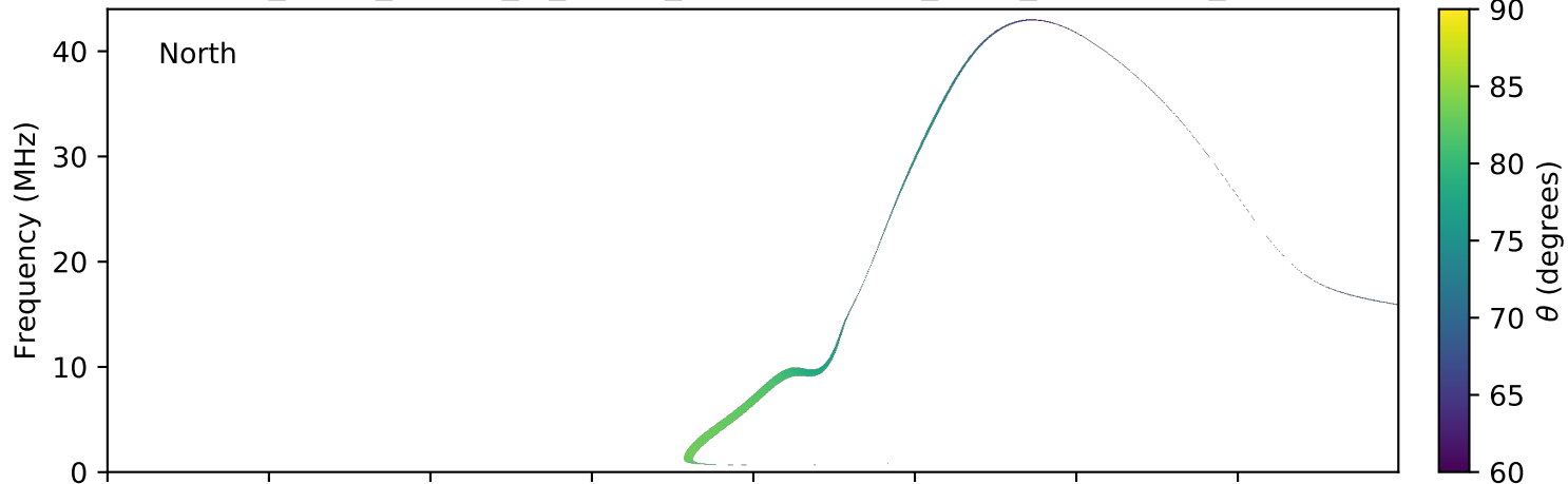
expres_earth_jupiter_io_jrm09_lossc-wid1deg_3kev_20181010_v01.cdf
