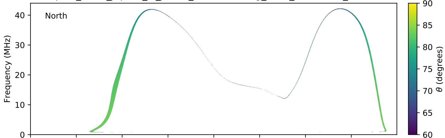
expres_earth_jupiter_io_jrm09_lossc-wid1deg_3kev_20181005_v01.cdf
