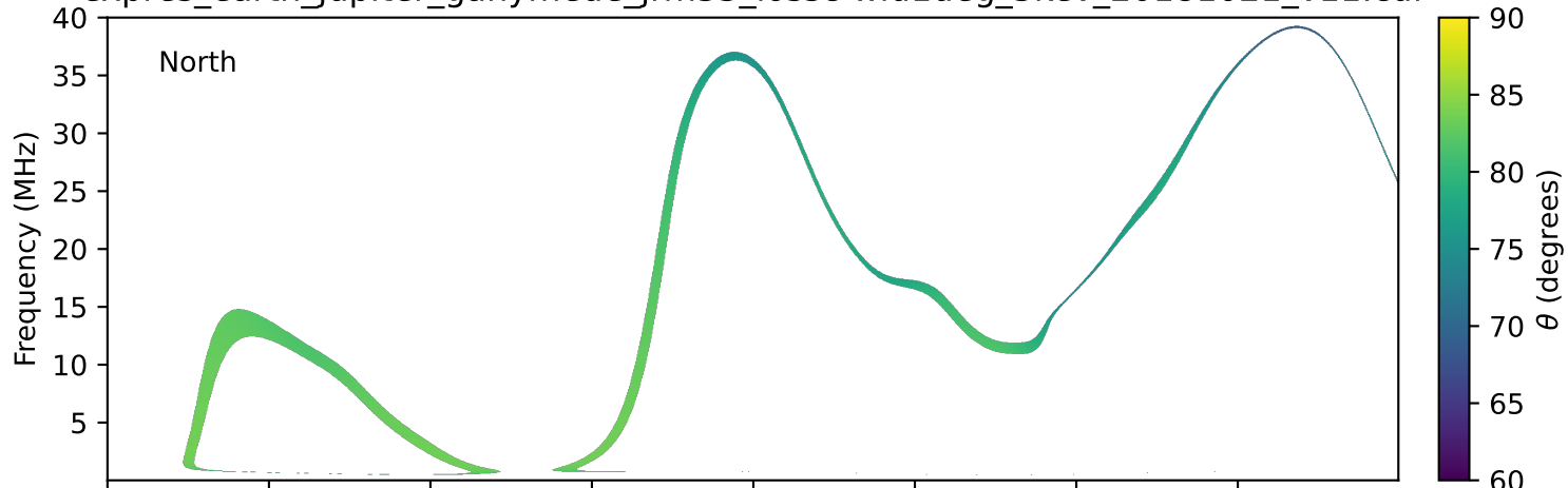
expres_earth_jupiter_ganymede_jrm33_lossc-wid1deg_3kev_20181021_v11.cdf
