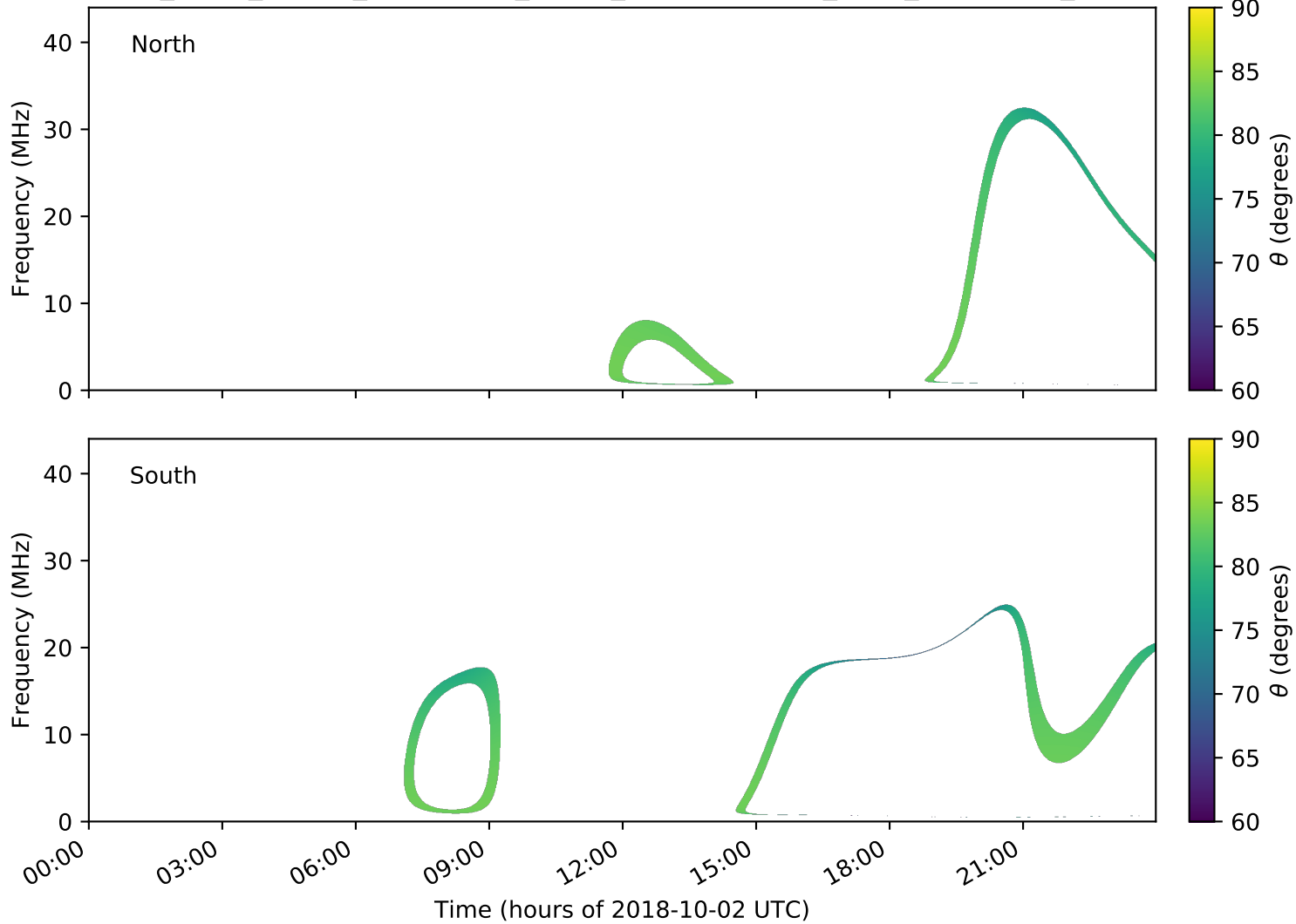
expres_earth_jupiter_ganymede_jrm09_lossc-wid1deg_3kev_20181002_v01.cdf
