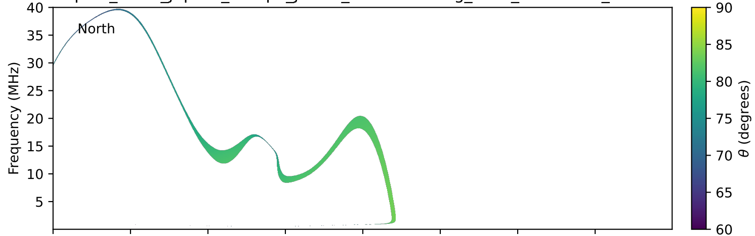
expres_earth_jupiter_europa_jrm33_lossc-wid1deg_3kev_20181019_v11.cdf
