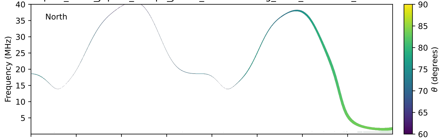
expres_earth_jupiter_europa_jrm33_lossc-wid1deg_3kev_20181001_v11.cdf
