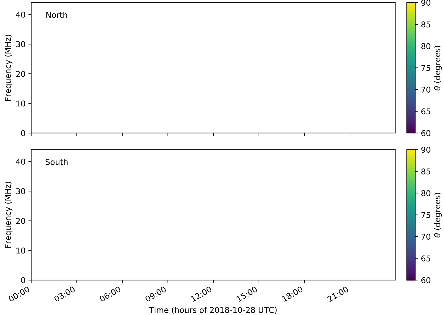
expres_earth_jupiter_europa_jrm09_lossc-wid1deg_3kev_20181028_v01.cdf
