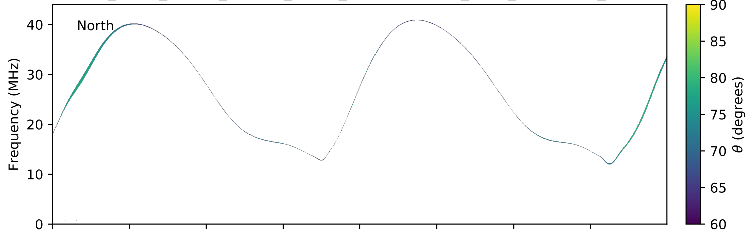
expres_earth_jupiter_europa_jrm09_lossc-wid1deg_3kev_20181023_v01.cdf
