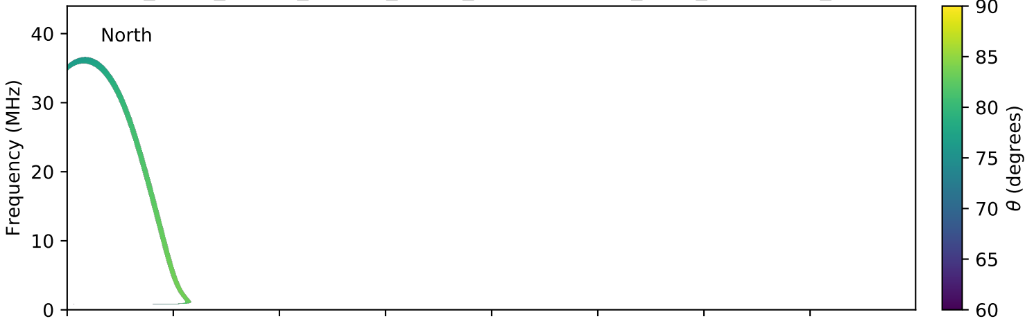
expres_earth_jupiter_europa_jrm09_lossc-wid1deg_3kev_20181017_v01.cdf
