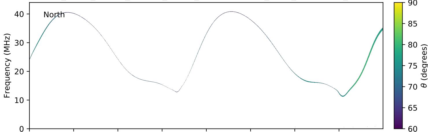
expres_earth_jupiter_europa_jrm09_lossc-wid1deg_3kev_20181016_v01.cdf
