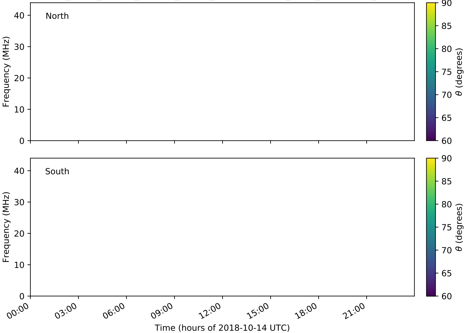
expres_earth_jupiter_europa_jrm09_lossc-wid1deg_3kev_20181014_v01.cdf
