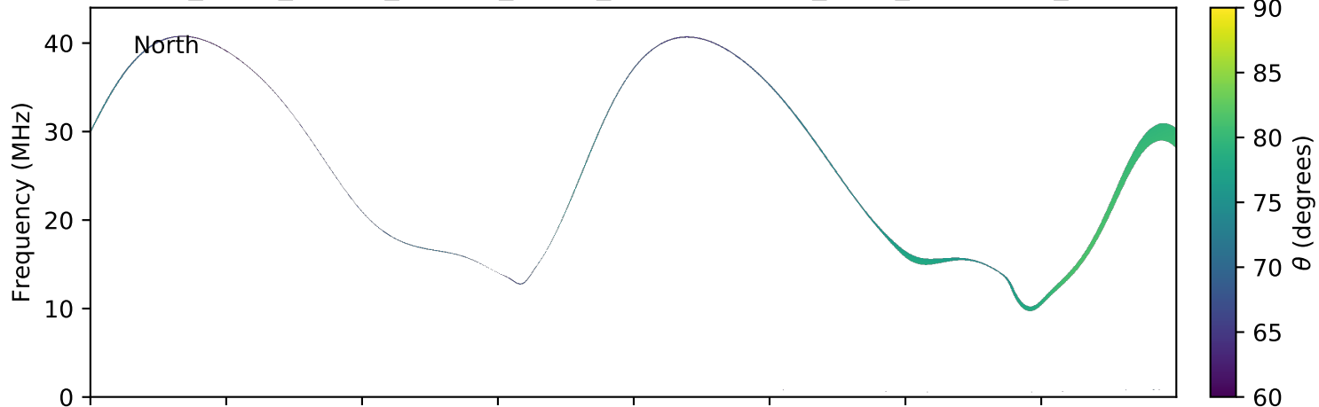
expres_earth_jupiter_europa_jrm09_lossc-wid1deg_3kev_20181009_v01.cdf
