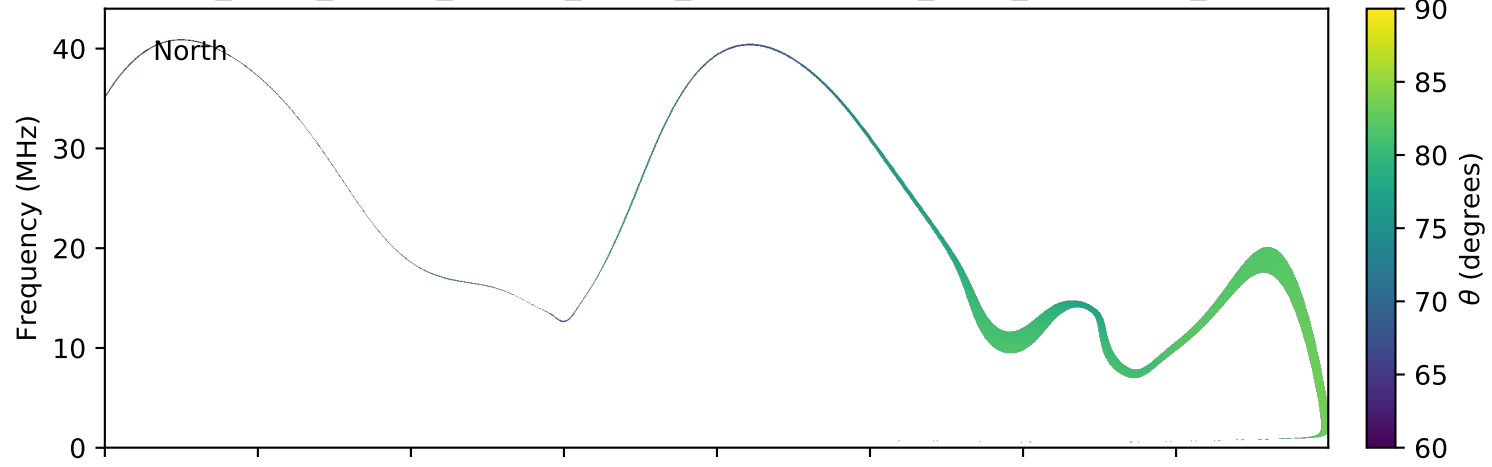
expres_earth_jupiter_europa_jrm09_lossc-wid1deg_3kev_20181002_v01.cdf
