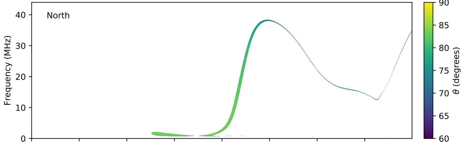
expres_earth_jupiter_europa_jrm09_lossc-wid1deg_3kev_20181001_v01.cdf
