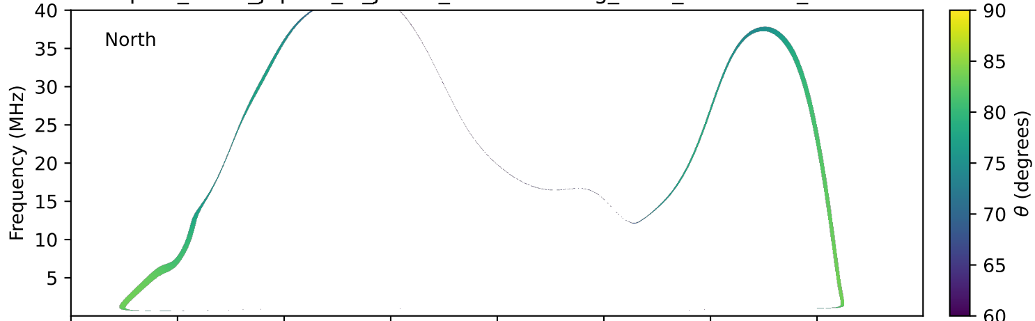
expres_earth_jupiter_io_jrm33_lossc-wid1deg_3kev_20180928_v11.cdf
