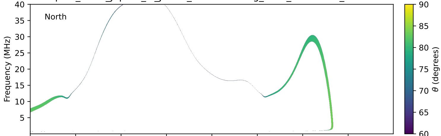
expres_earth_jupiter_io_jrm33_lossc-wid1deg_3kev_20180921_v11.cdf
