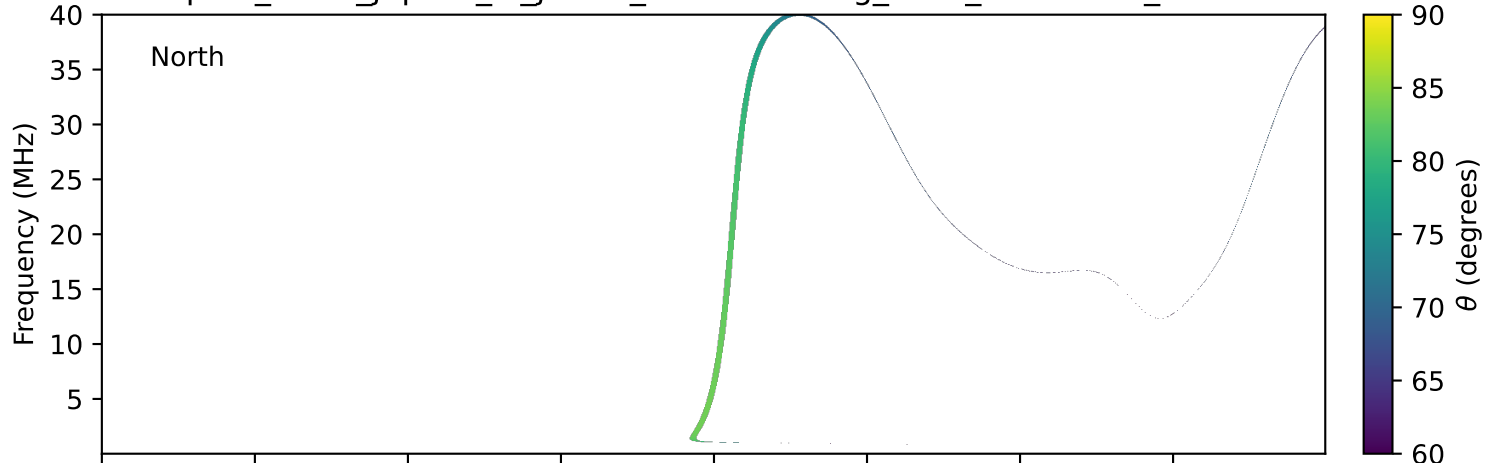
expres_earth_jupiter_io_jrm33_lossc-wid1deg_3kev_20180917_v11.cdf
