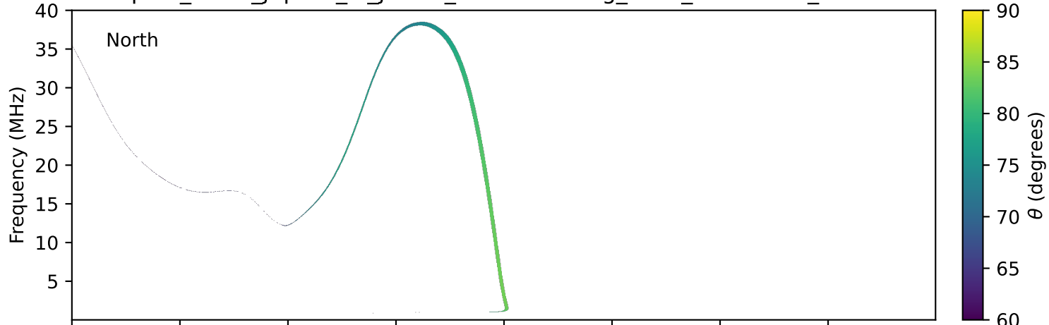
expres_earth_jupiter_io_jrm33_lossc-wid1deg_3kev_20180916_v11.cdf
