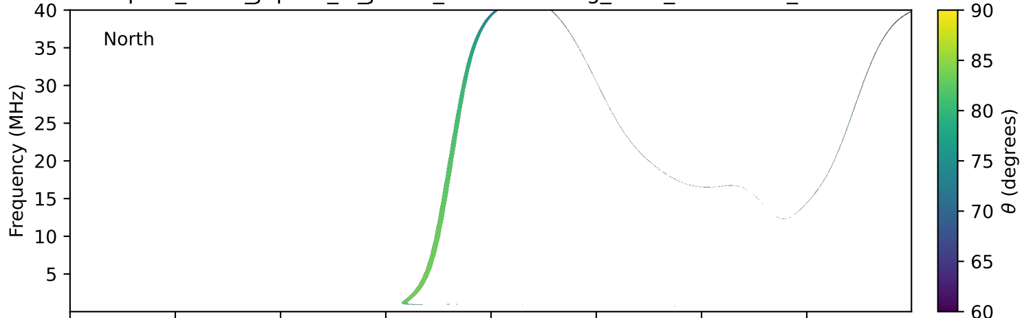
expres_earth_jupiter_io_jrm33_lossc-wid1deg_3kev_20180910_v11.cdf
