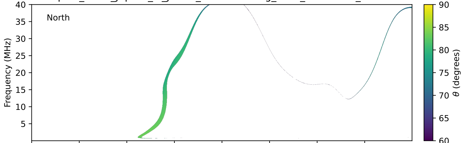
expres_earth_jupiter_io_jrm33_lossc-wid1deg_3kev_20180903_v11.cdf
