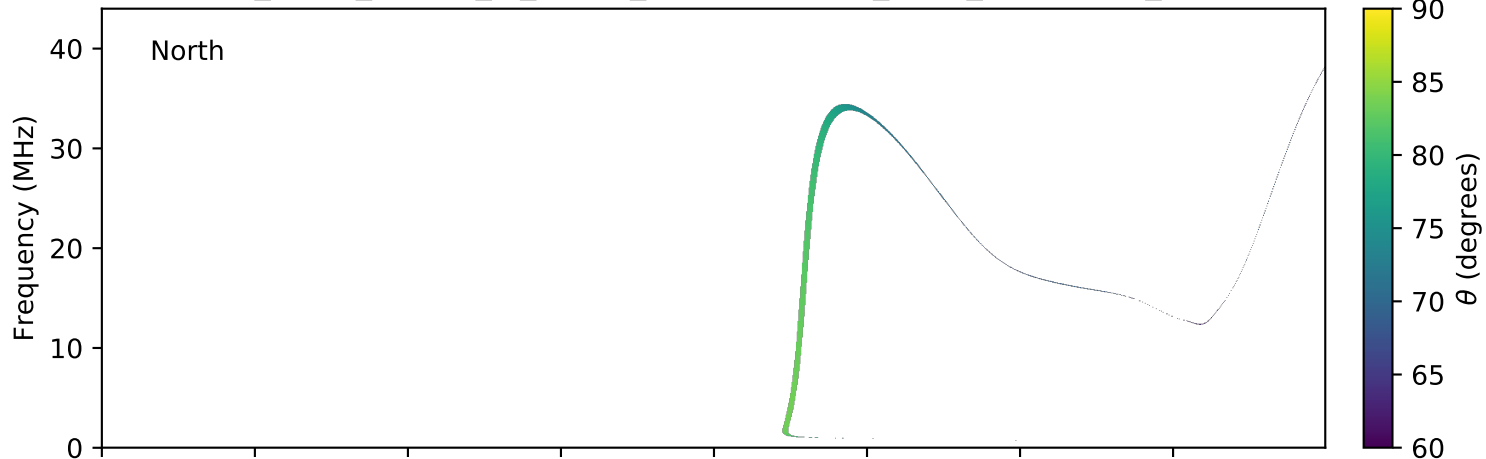
expres_earth_jupiter_io_jrm09_lossc-wid1deg_3kev_20180924_v01.cdf
