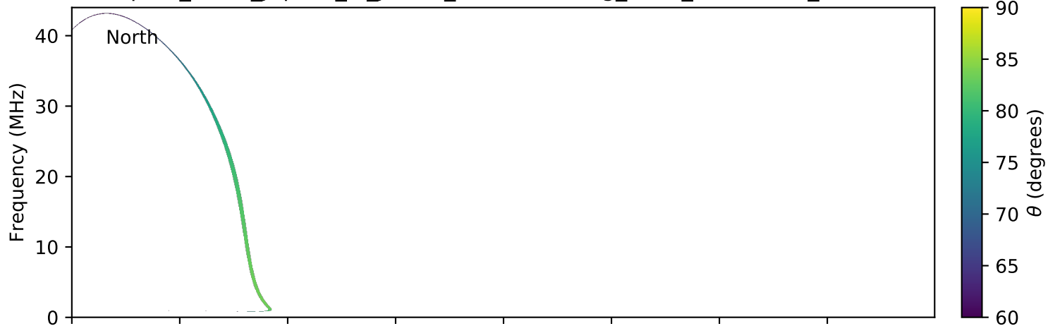
expres_earth_jupiter_io_jrm09_lossc-wid1deg_3kev_20180918_v01.cdf
