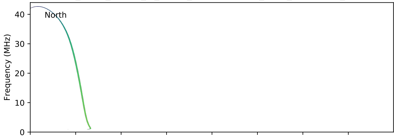
expres_earth_jupiter_io_jrm09_lossc-wid1deg_3kev_20180911_v01.cdf
