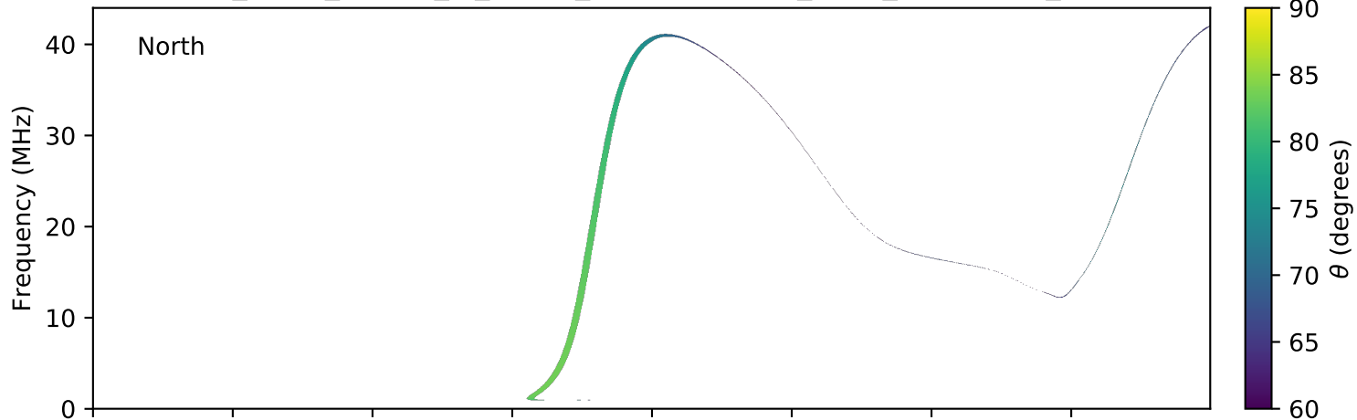
expres_earth_jupiter_io_jrm09_lossc-wid1deg_3kev_20180910_v01.cdf
