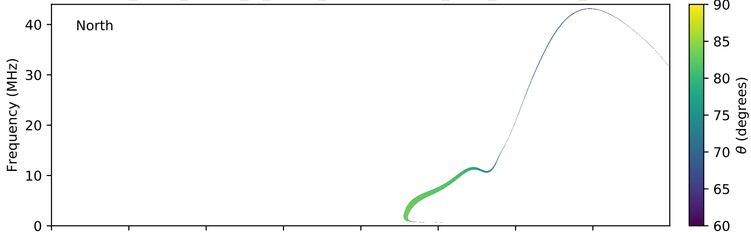
expres_earth_jupiter_io_jrm09_lossc-wid1deg_3kev_20180908_v01.cdf
