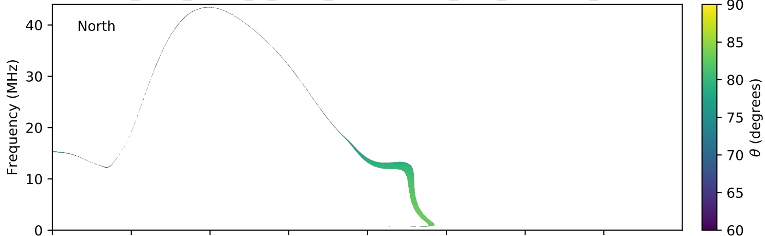
expres_earth_jupiter_io_jrm09_lossc-wid1deg_3kev_20180907_v01.cdf
