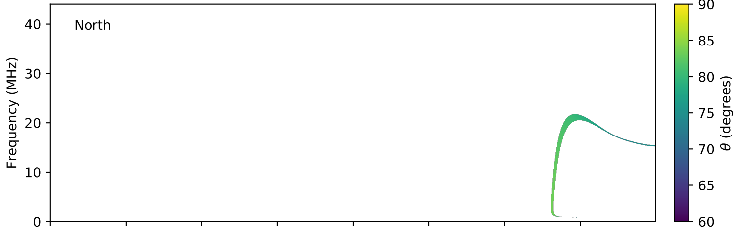
expres_earth_jupiter_io_jrm09_lossc-wid1deg_3kev_20180906_v01.cdf
